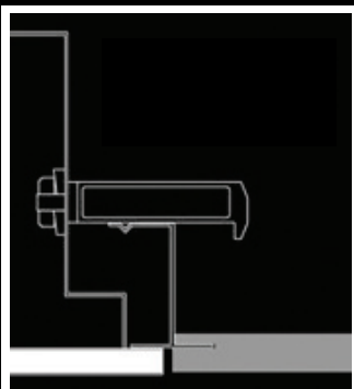
Concealed T Bar Ceiling Mounted in a Concealed T bar ceiling, pushed up from below
