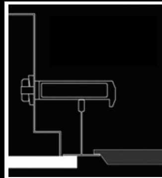
T Bar Ceiling Mounted in a T bar ceiling, pushed up from below
